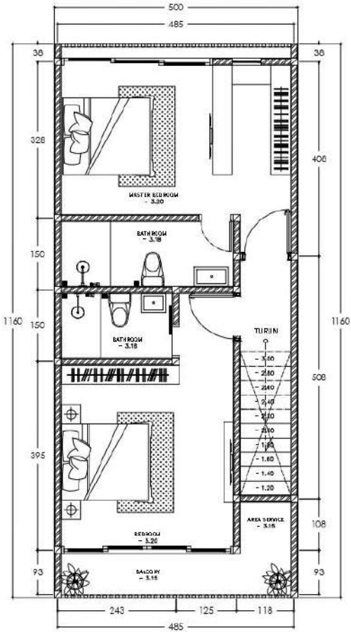
DENAH LANTAI 3 SCALE 1 : 100
