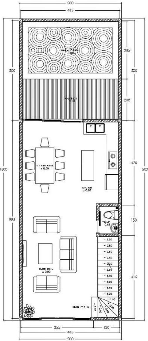
DENAH LANTAI 1 SCALE 1 : 100
