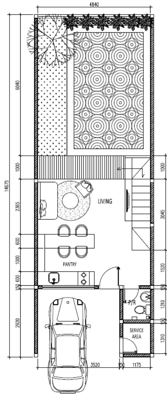
FURNITURE LAYOUT PLAN - ENZIO TYPE 1 (2 BEDROOM)
